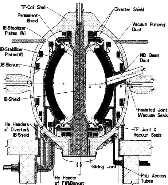
Fig. 1. Vertical cross-section of ARIES-ST
