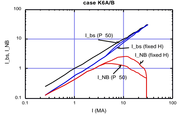
Fig. 6. Current ramp during startup on ARIES-ST.
