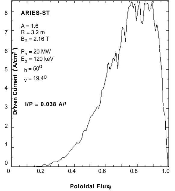
Fig.4. Off-axis neutral beam CD in ASRIES-ST.
