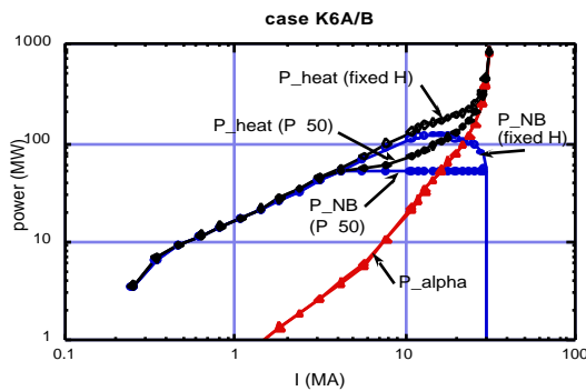
Fig. 5. Power input during startup on ARIES-ST.
