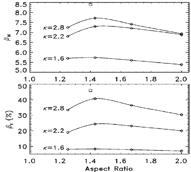
Fig. 1. Ballooning stability limits for 99% bootstrapped ST equilibria for various A and \kappa , and at fixed \delta . [4] The square point is for optimized pressure profile at \kappa=2.8
