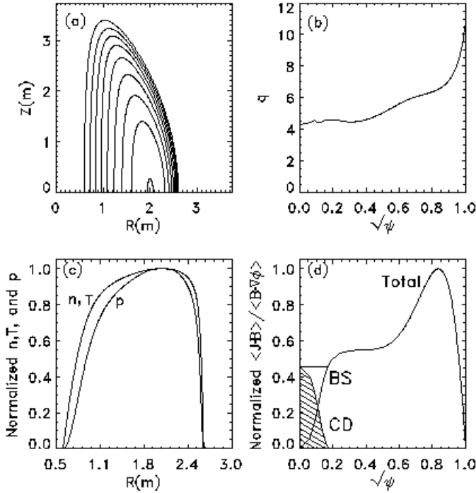
Fig. 3. Reference equilibrium for ARIES-ST.
