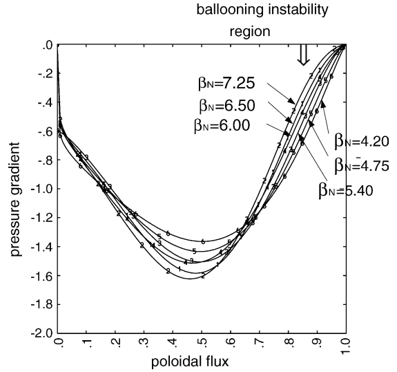
Fig. 4. A series of pressure gradient profiles as a function of poloidal flux showing how the gradient is reduced in the ballooning unstable region to obtain successively higher \beta_N values, while keeping bootstrap alignment.
